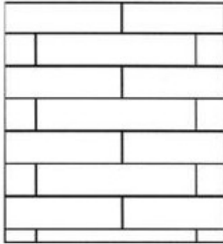
Avoid H Joints
